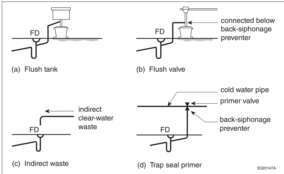
Figure A-2.4.5.5.(1) Maintaining trap seals
