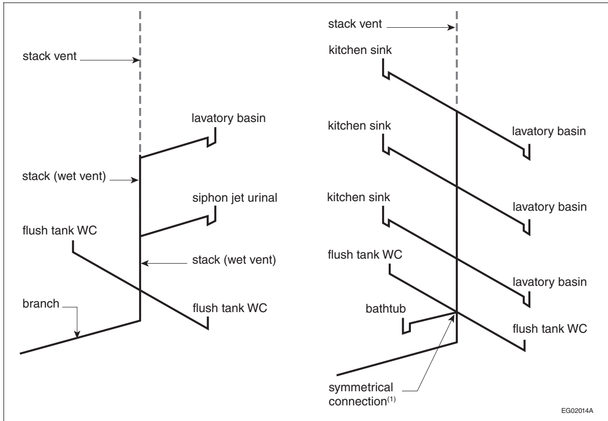
Figure A-2.5.2.1-B Example of wet venting described in Clause 2.5.2.1.(1)(c)
