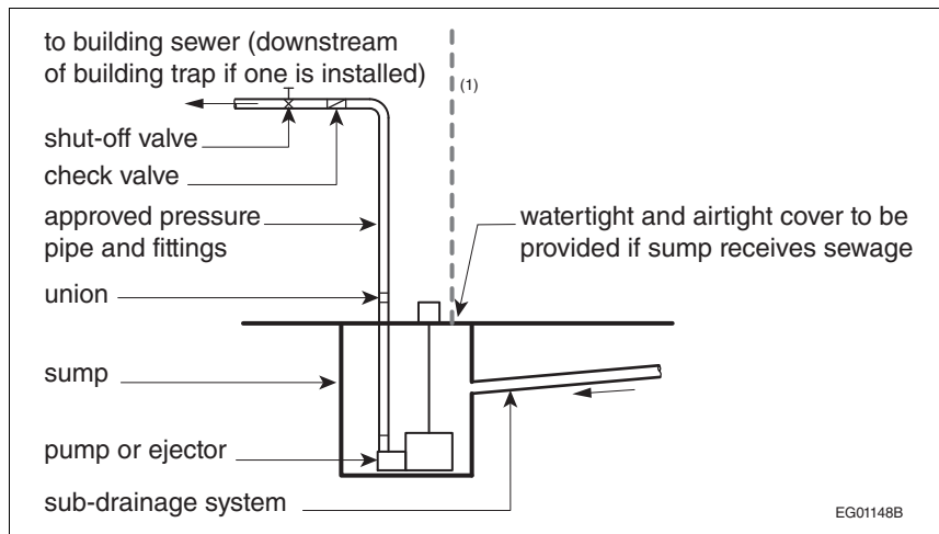
Figure A-2.4.6.3. Arrangement of piping at sump
