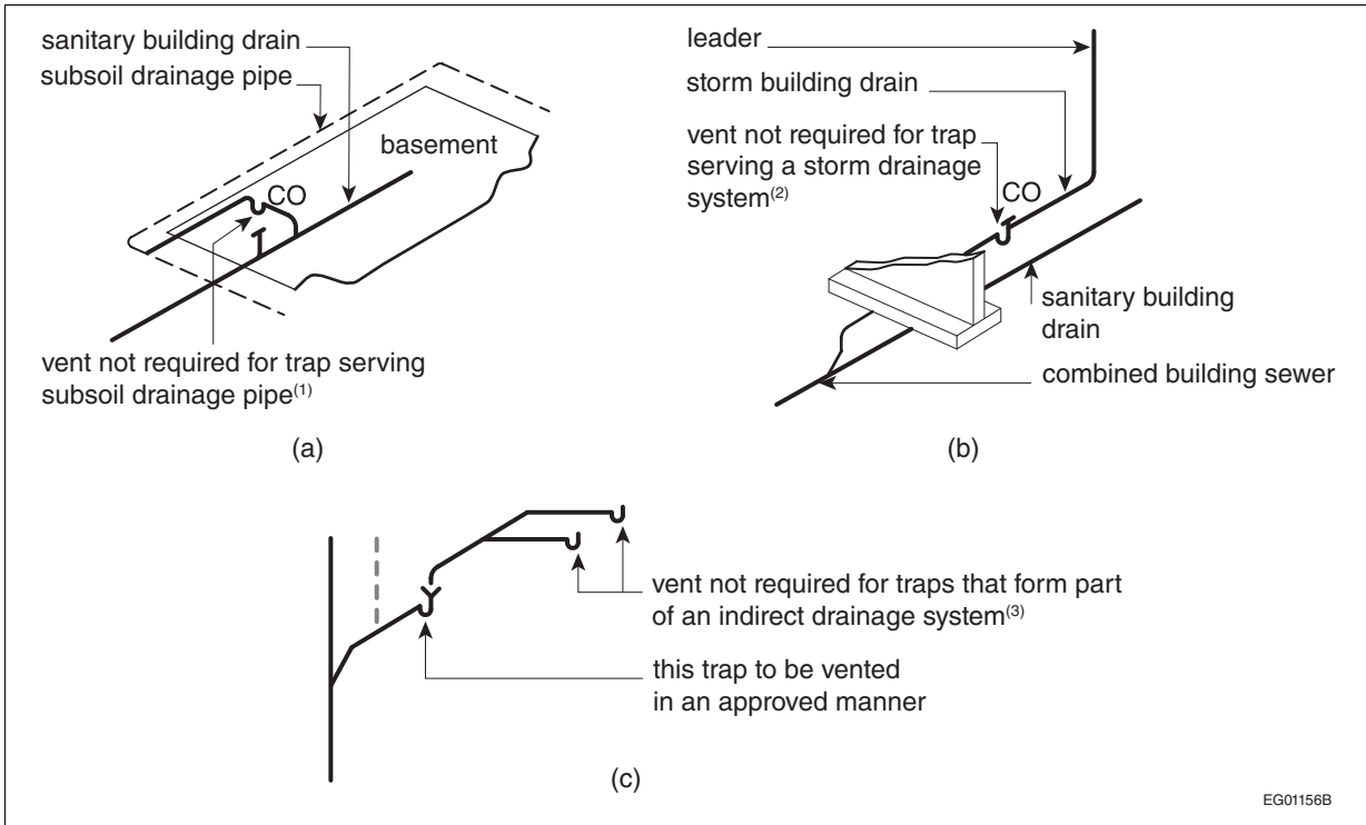
Figure A-2.5.1.1.(4) Venting not required
