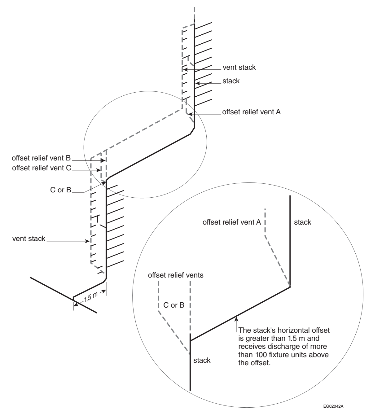
Figure A-2.5.4.4.(1) Offset relief vents
