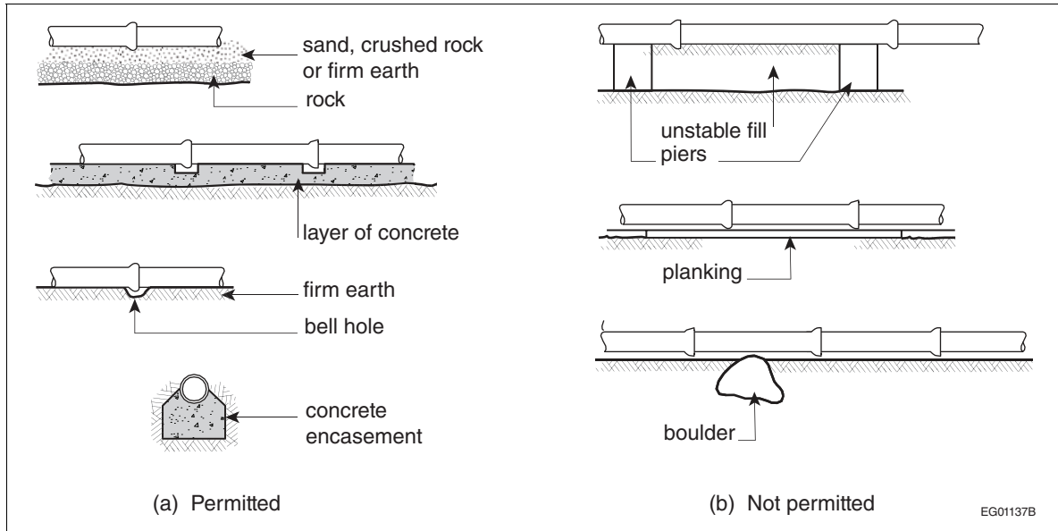
Figure A-2.3.4.6.(1) Support for underground piping
