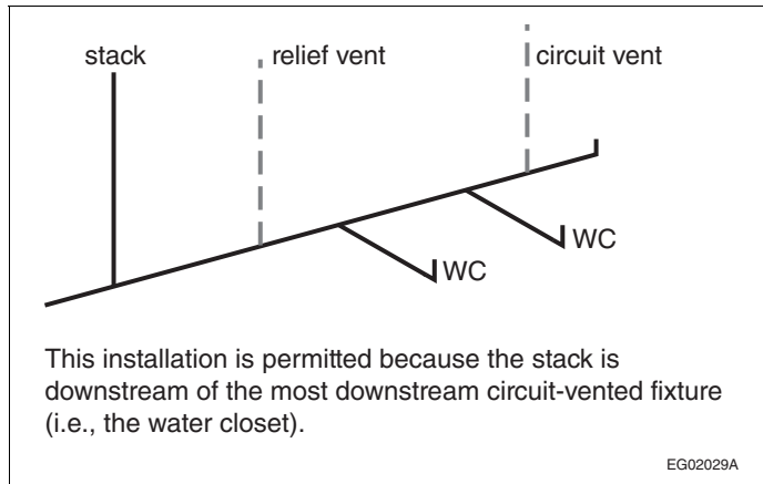
Figure A-2.5.3.1.-B Example of circuit venting described in Clause 2.5.3.1.(1)(c)
