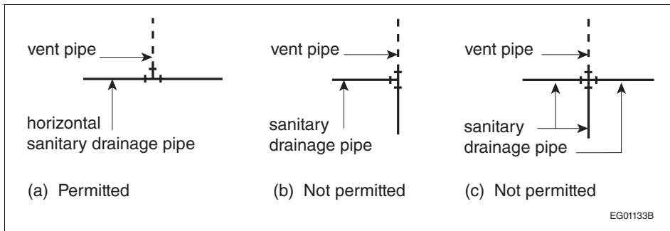
Figure A-2.2.4.1. T fittings in drainage systems
