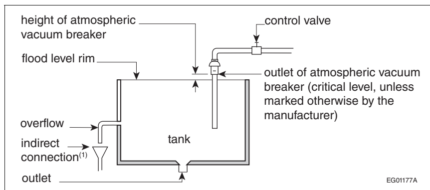
Figure A-2.6.2.10.(2) Installation of atmospheric vacuum breakers
