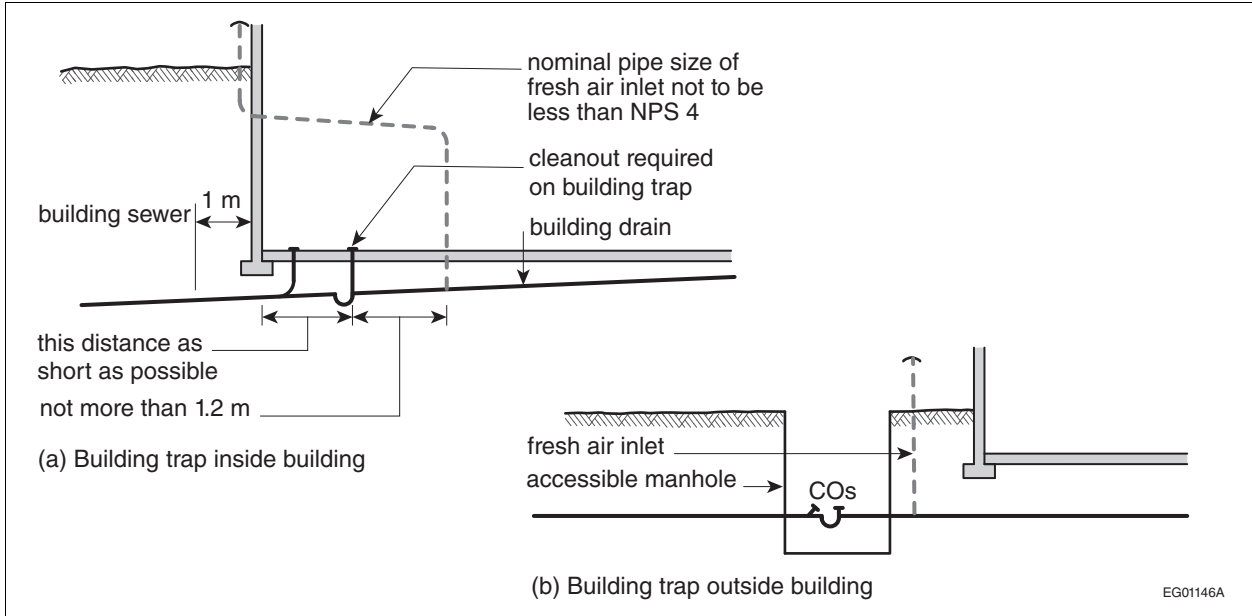
Figure A-2.4.5.4.(1) Location of building traps
