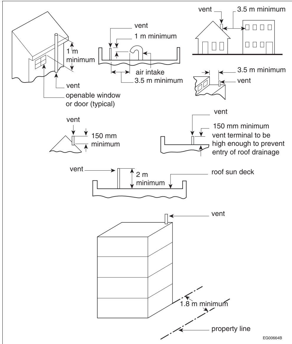
Figure A-2.5.6.5.(4) Vent terminals
