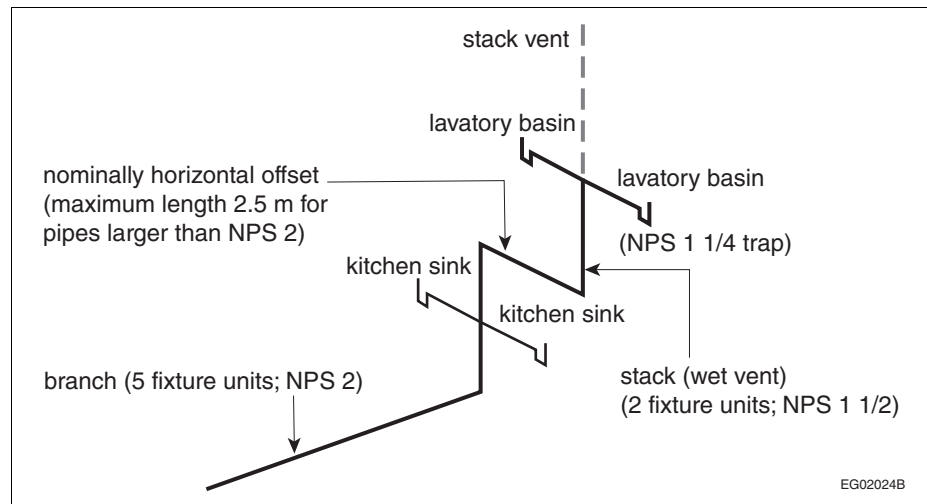
Figure A-2.5.2.1.-K Example of wet venting described in Subclause 2.5.2.1.(1)(i)(ii)
