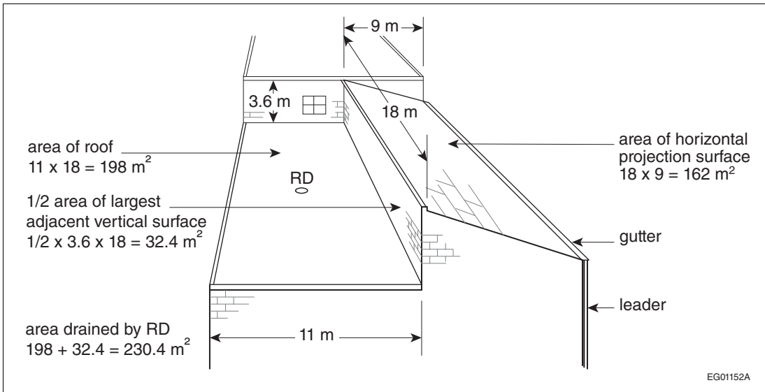
Figure 1-1 Storm drainage areas (example 1)
