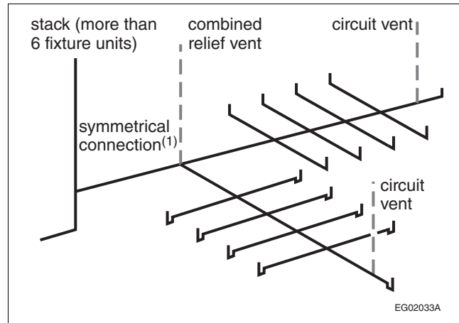
Figure A-2.5.3.1.-F Example of circuit venting described in Sentence 2.5.3.1.(5)
