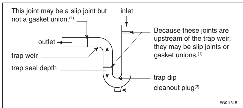
Figure A-2.2.3.1.(1) and (3) Trap seal depth and trap connections
