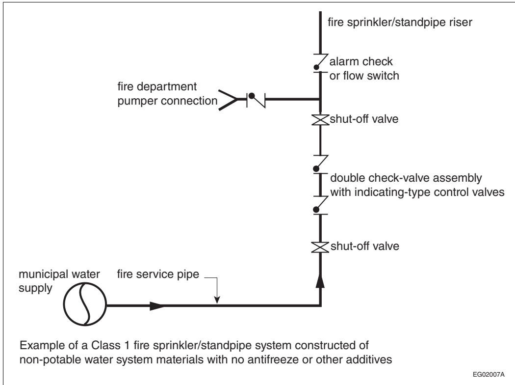
Figure A-2.6.2.4.(3) Fire department pumper connection and backflow protection
