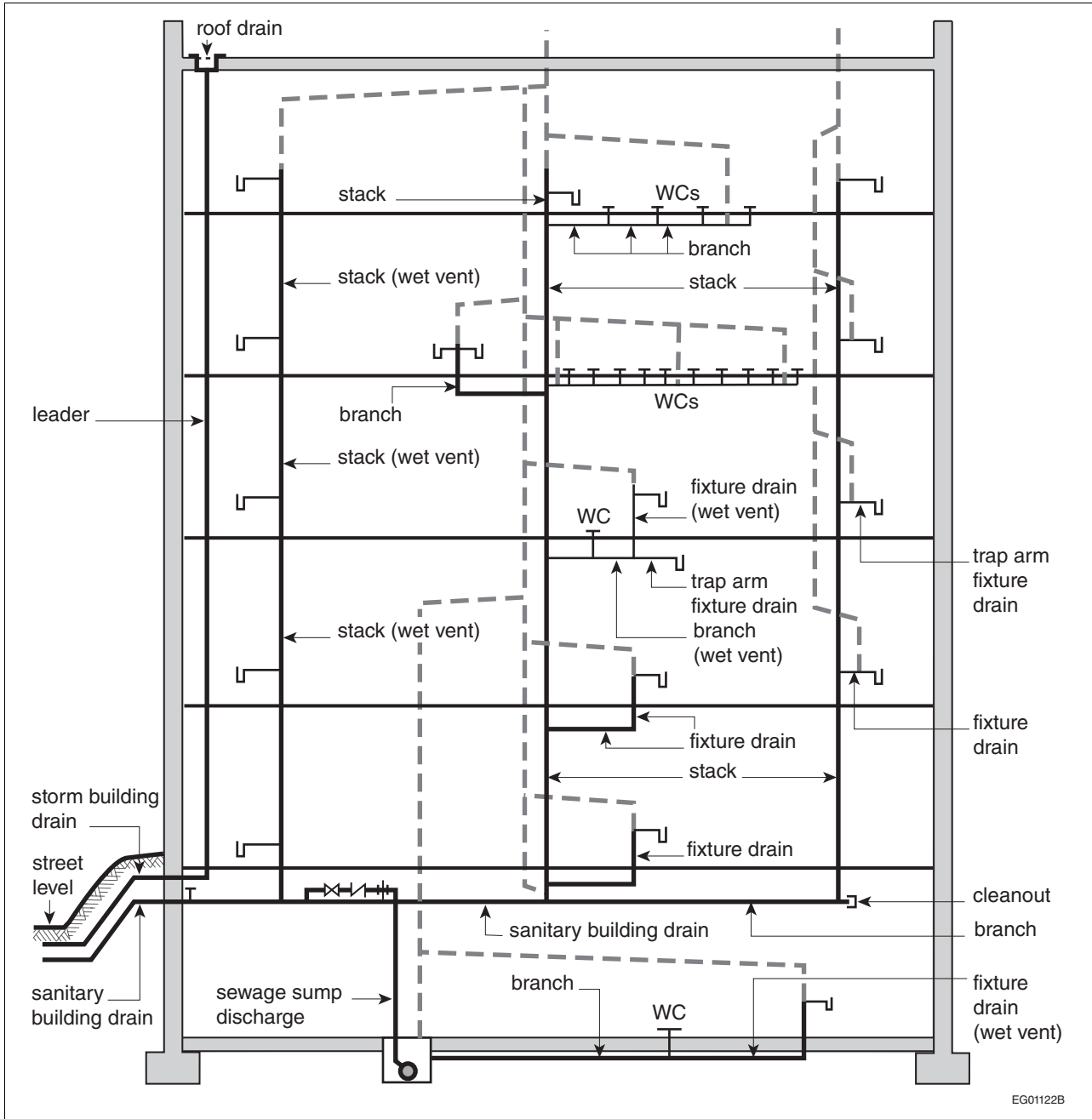
Figure A-1.4.1.2.(1)-F Drainage system
