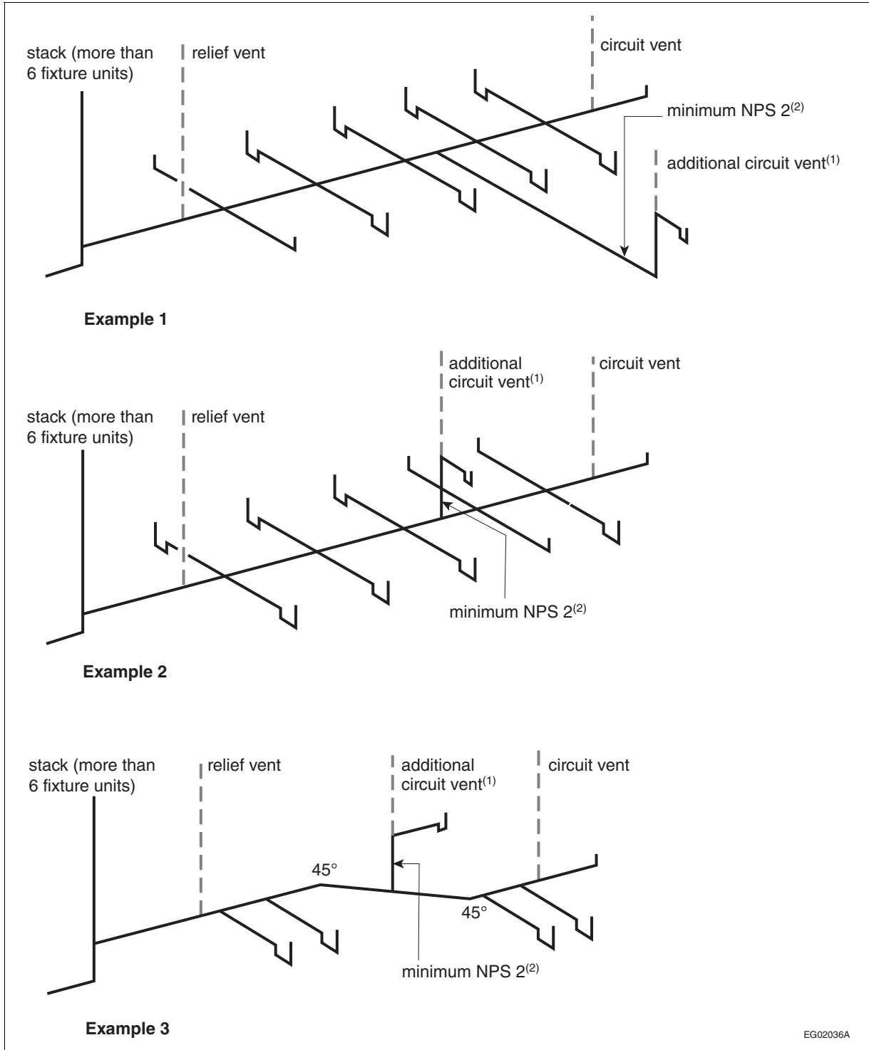
Figure A-2.5.3.1.-I Example of circuit venting described in Sentence 2.5.3.1.(7)
