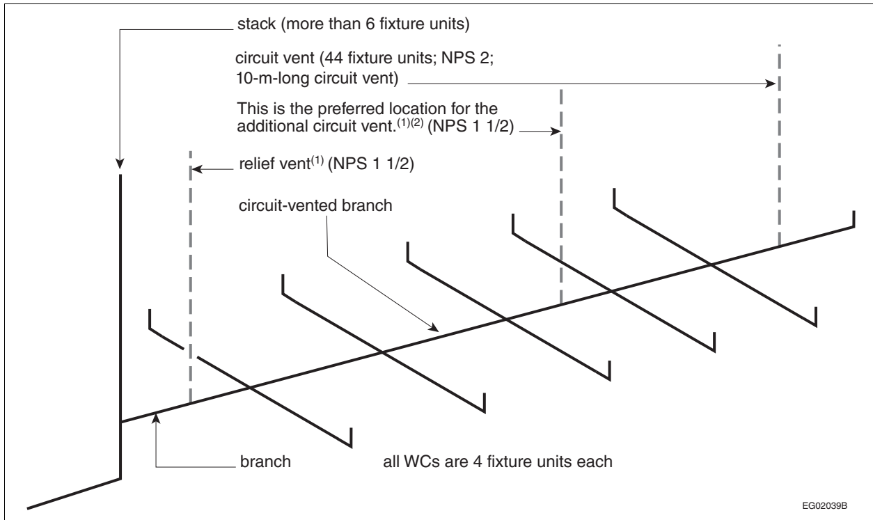
Figure A-2.5.3.1.-L
