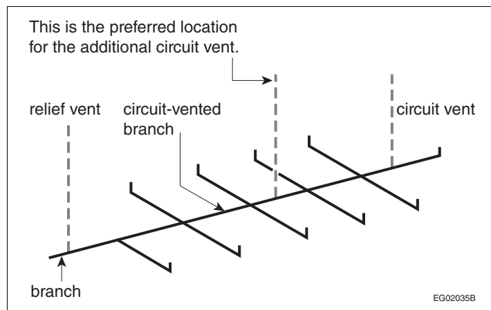
Figure A-2.5.3.1.-H Example of circuit venting described in Clause 2.5.3.1.(6)(b)
