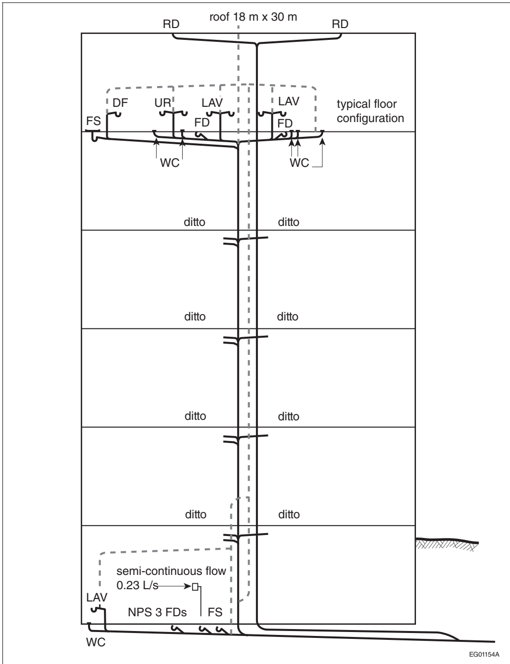
Figure 2-1 Building drainage system (example 2)
