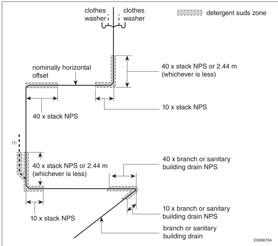
Figure A-2.4.2.1.(4) and (5) Suds pressure zones
