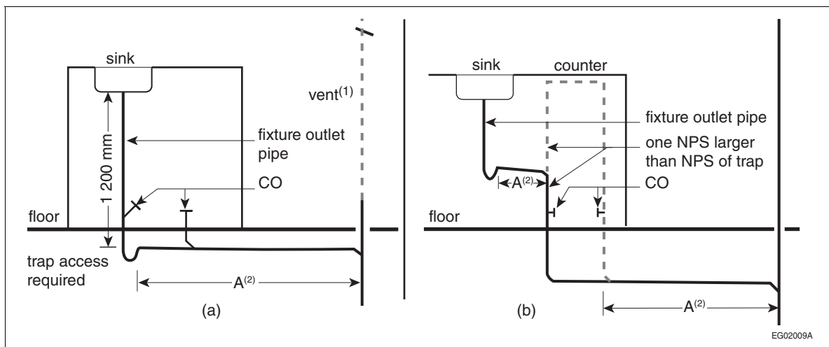
Figure A-2.4.8.2.(1) Island fixture installation (3)
