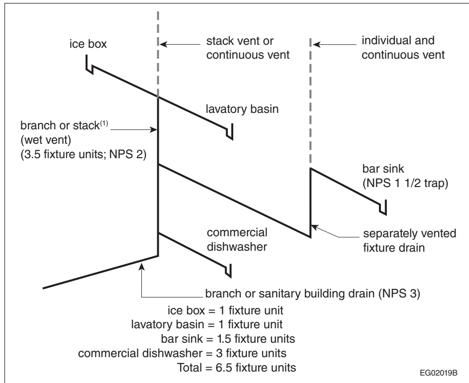
Figure A-2.5.2.1-G Example of wet venting described in Clause 2.5.2.1.(1)(f)
