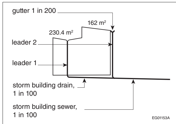
Figure 1-2 Storm drainage components (example 1) (elevation view)
