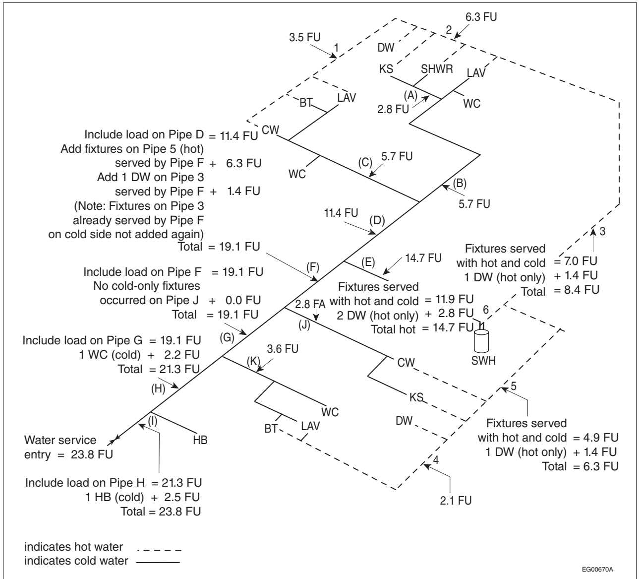
Figure A-2.6.3.4.(5)-B Example of water pipe sizing for buildings containing one or two dwelling units or row houses with separate water services
