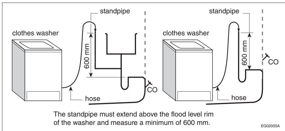
Figure A-2.4.9.3.(3) Standpipe installation for clothes washers
