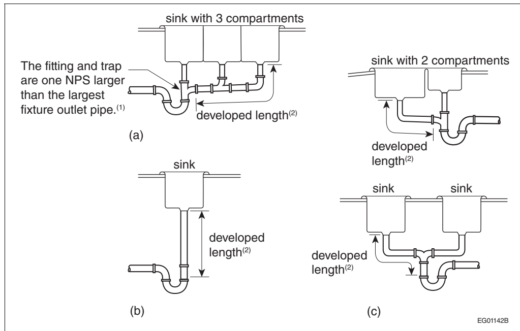
Figure A-2.4.5.1.(2) Trapping of sinks and laundry trays
