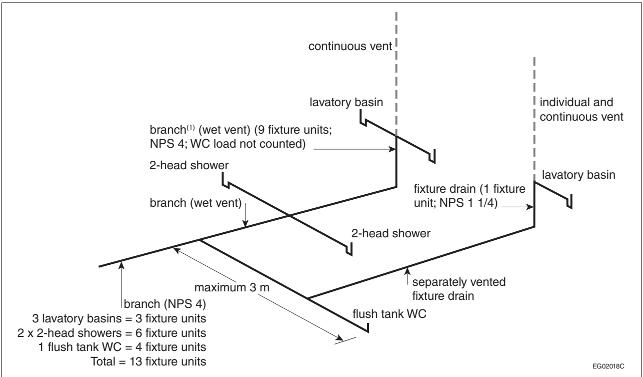
Figure A-2.5.2.1-F Example of wet venting described in Clause 2.5.2.1.(1)(f)
