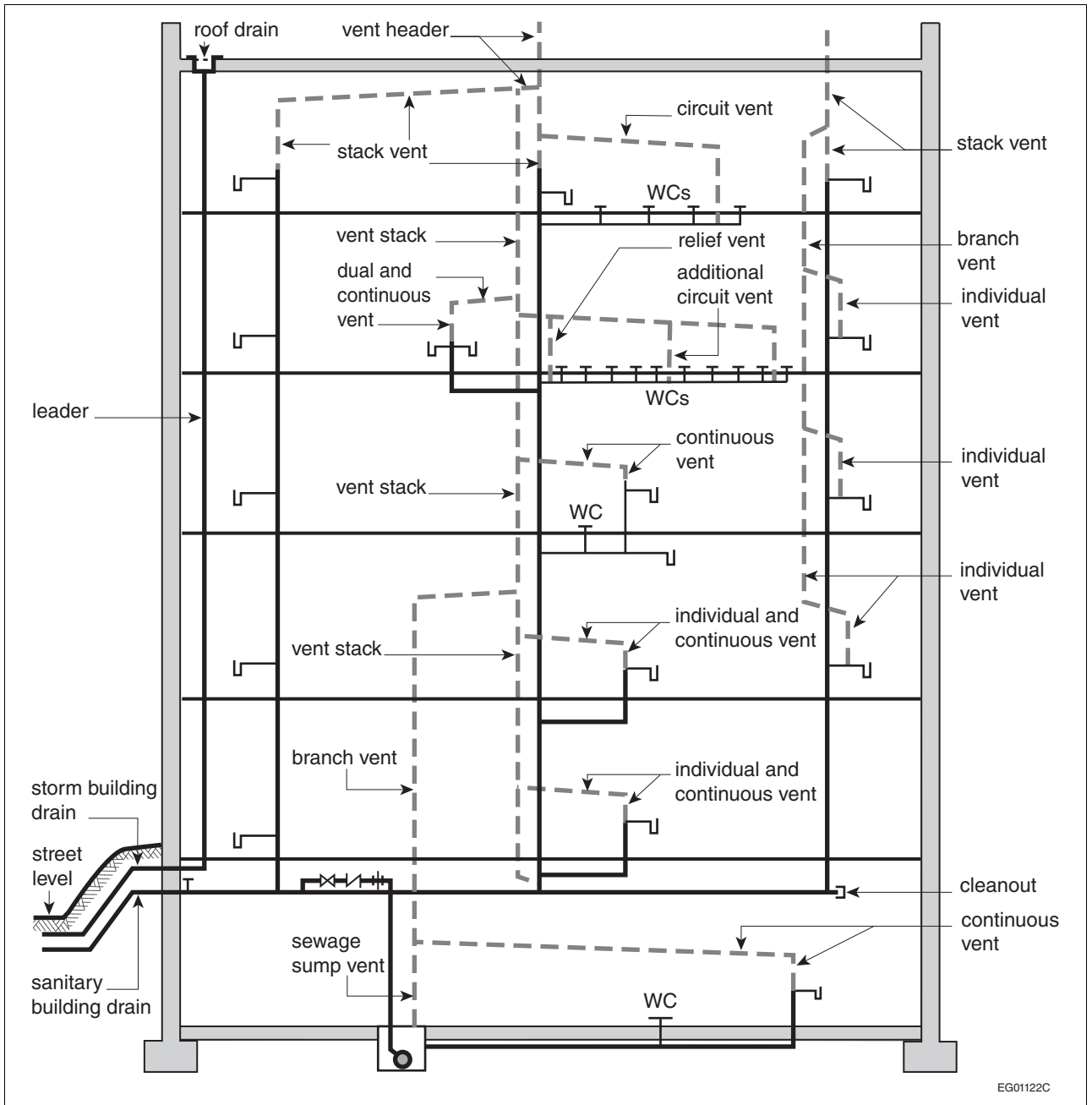
Figure A-1.4.1.2.(1)-G Venting system
