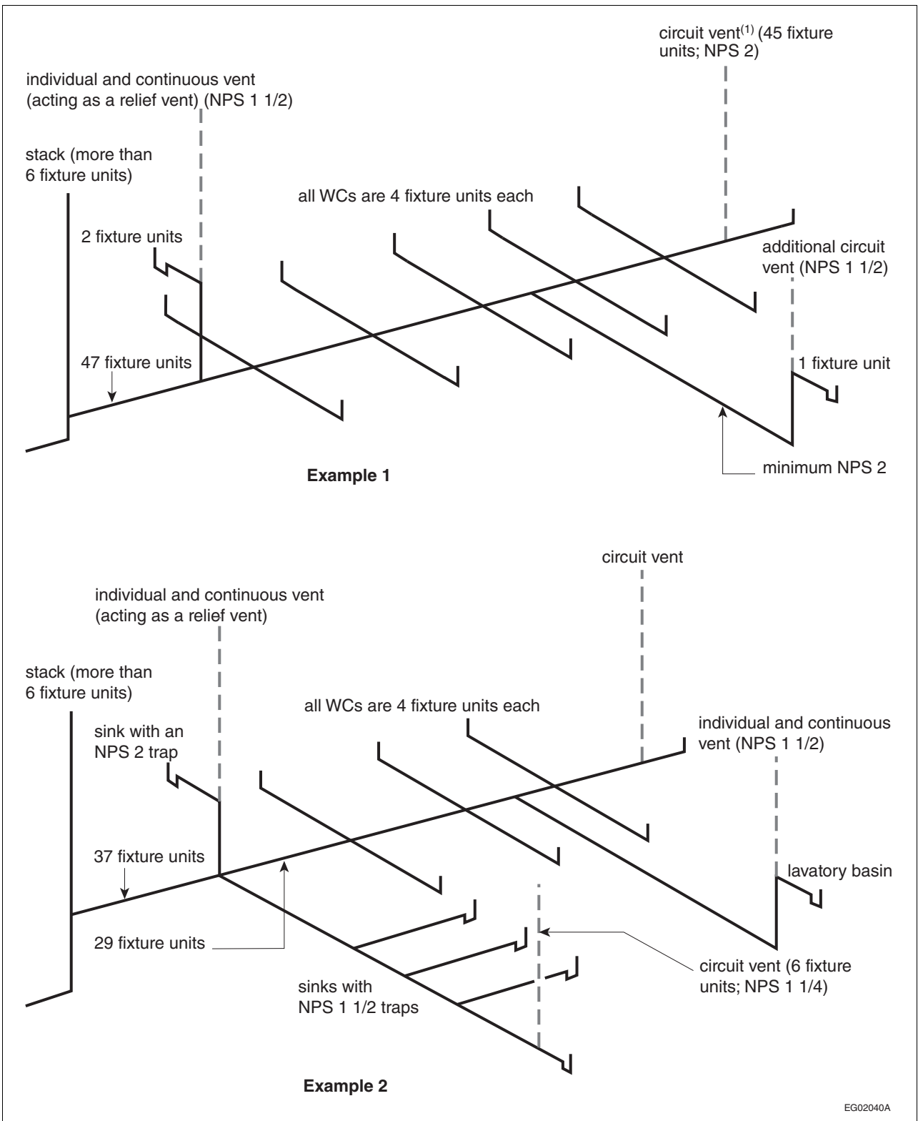
Figure A-2.5.3.1.-M Example of circuit venting described in Sentence 2.5.3.1.(11)
