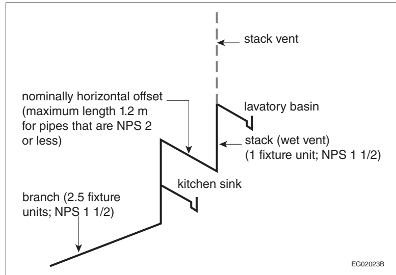
Figure A-2.5.2.1.-J Example of wet venting described in Subclause 2.5.2.1.(1)(i)(i)
