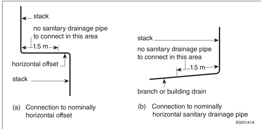
Figure A-2.4.2.1.(2) Sanitary drainage pipe connections
