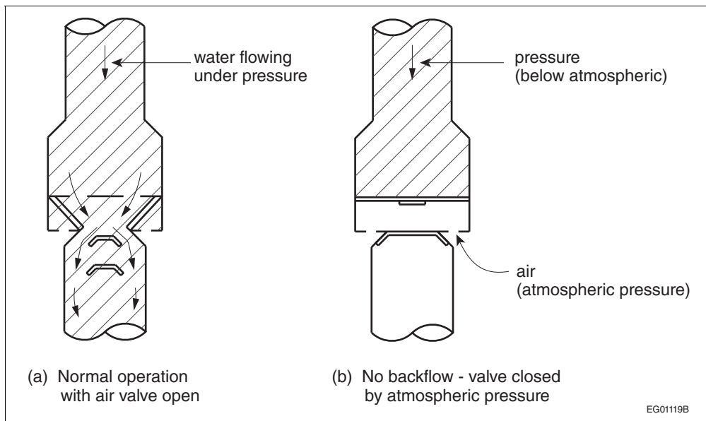
Figure A-1.4.1.2.(1)-C
