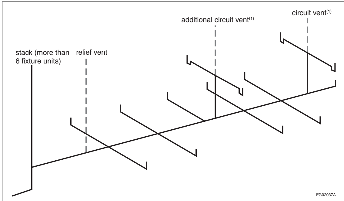
Figure A-2.5.3.1.-J Example of circuit venting described in Sentence 2.5.3.1.(8)
