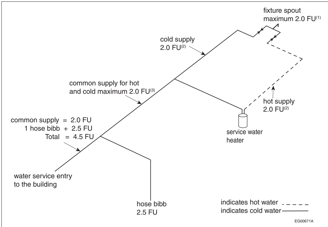
Figure A-2.6.3.4.(5)-A Determining the hydraulic needs of a fixture
