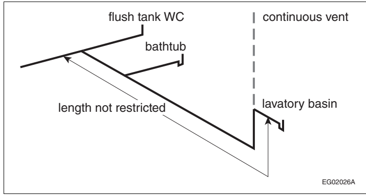
Figure A-2.5.2.1.-M Example of wet venting described in Clause 2.5.2.1.(1)(k)
