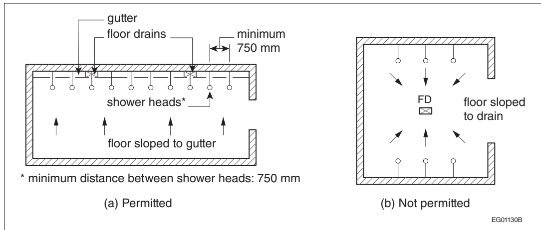
Figure A-2.2.2.3.(3) Shower drainage (plan view)
