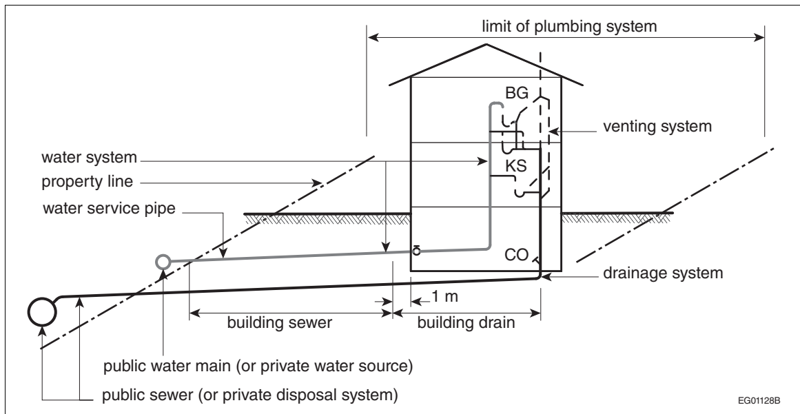
Figure A-1.4.1.2.(1)-L Plumbing system
