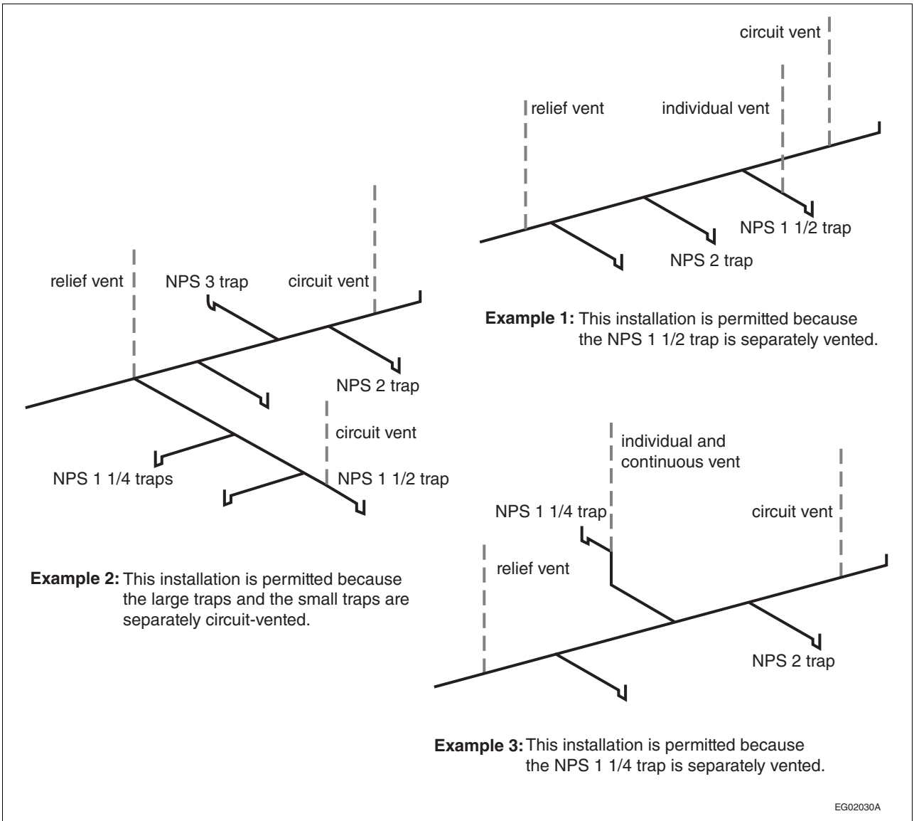
Figure A-2.5.3.1.-C Example of circuit venting described in Sentence 2.5.3.1.(2), which refers to the nominal pipe size of fixture outlets
