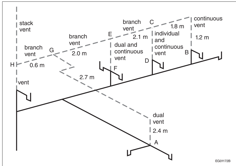
Figure A-2.5.8.3. and 2.5.8.4.-A Lengths to be considered when sizing branch, continuous, dual and individual vent pipes
