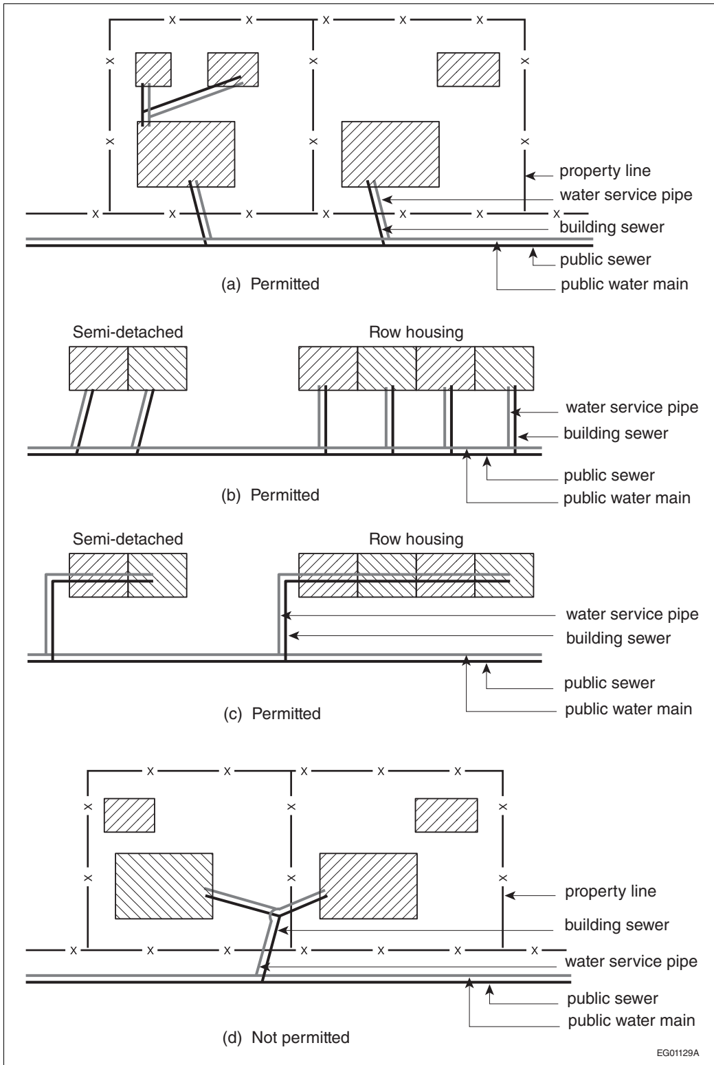
Figure A-2.1.2.4.(1) Service piping
