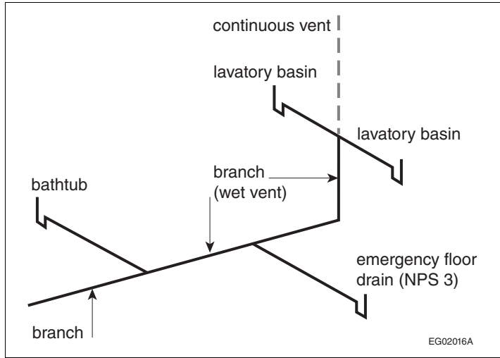
Figure A-2.5.2.1-D Example of wet venting described in Clause 2.5.2.1.(1)(e)
