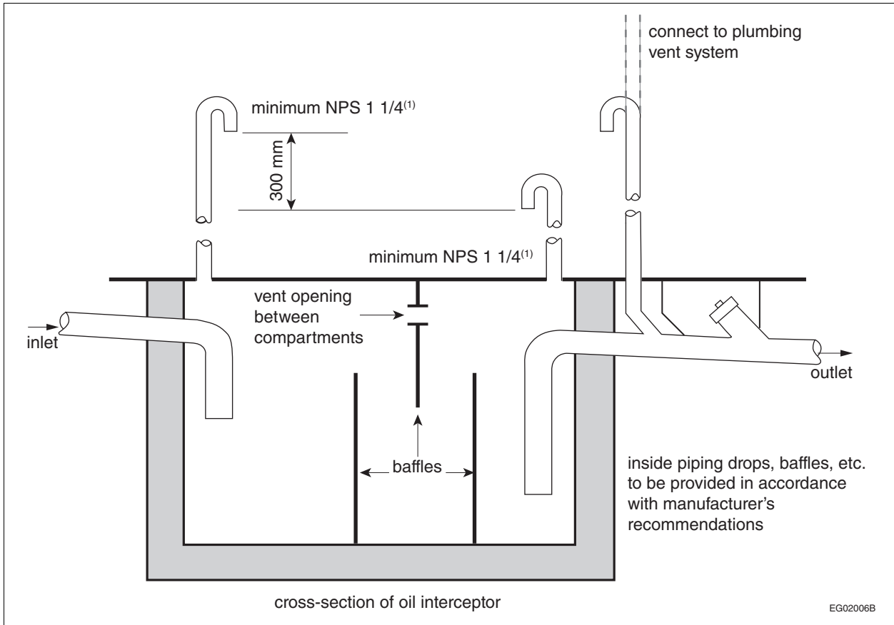
Figure A-2.5.5.2. Venting of oil interceptors
