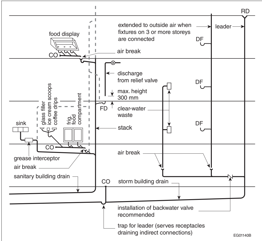
Figure A-2.4.2.1.(1)(a)(ii) and (e)(vi) Indirect connections
