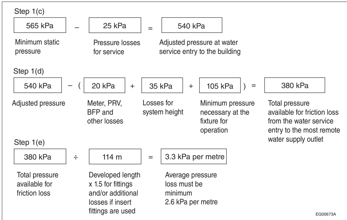
Figure A-2.6.3.1.(2)-B Determination of pressure available for friction loss
