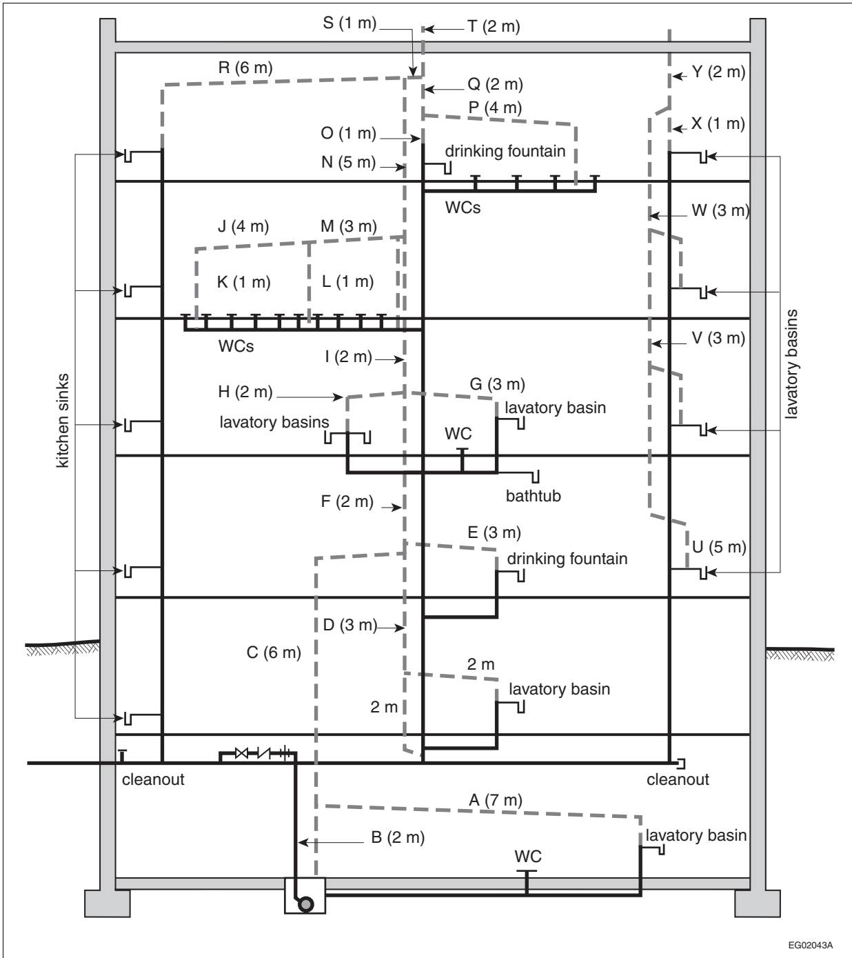
Figure A-2.5.8. Sizing of a venting system
