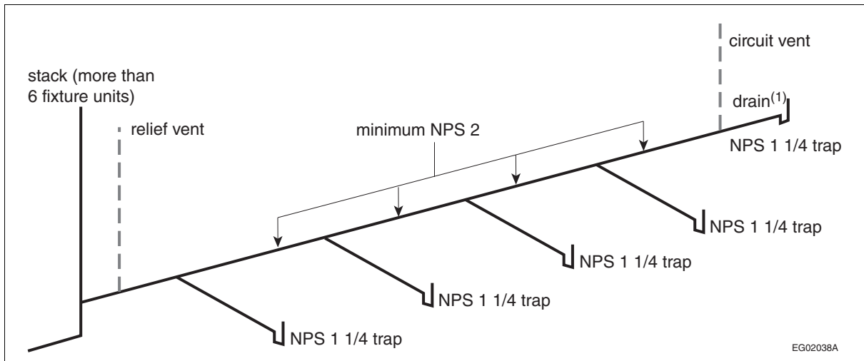
Figure A-2.5.3.1.-K Example of circuit venting described in Sentence 2.5.3.1.(9)
