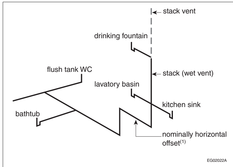
Figure A-2.5.2.1-I Example of wet venting described in Clause 2.5.2.1.(1)(i)
