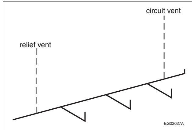
Figure A-2.5.3.1.-A Example of circuit venting described in Sentence 2.5.3.1.(1)
