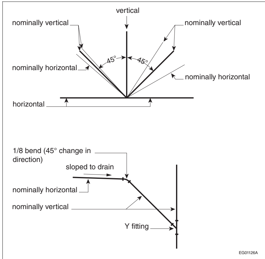
Figure A-1.4.1.2.(1)-J Nominally horizontal and nominally vertical
