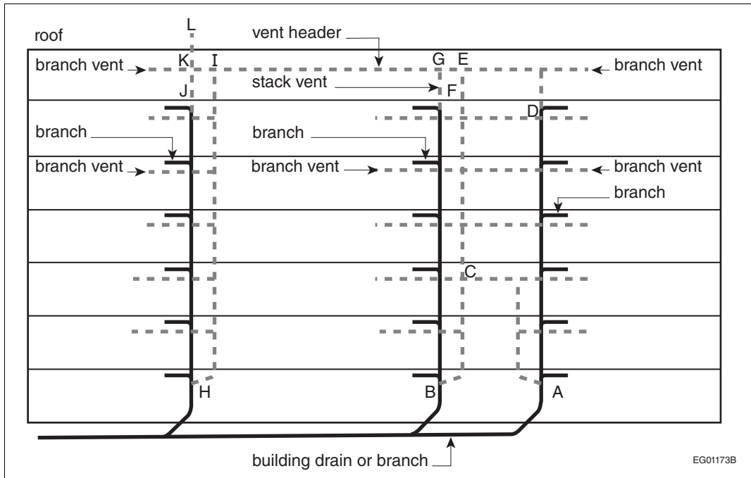
Figure A-2.5.8.3. and 2.5.8.4.-B Lengths to be considered when sizing stack vent, vent stack and vent header pipes
