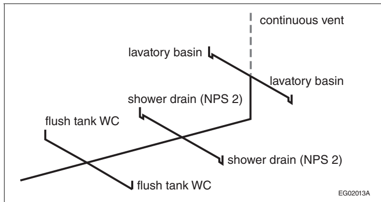
Figure A-2.5.2.1.-A Example of wet venting described in Clause 2.5.2.1.(1)(b)
