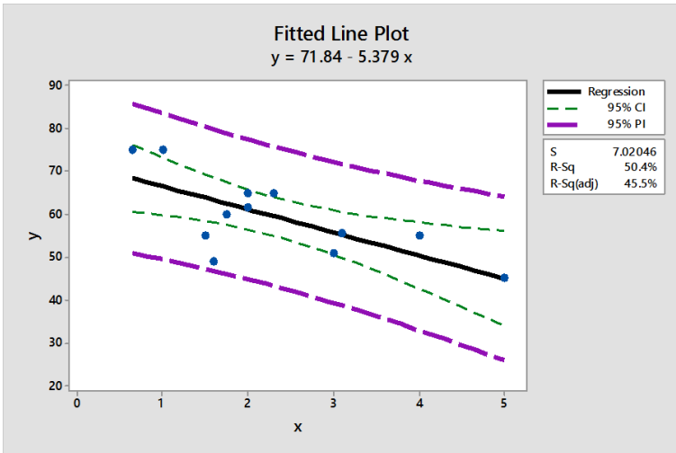
Figure 8.10 Minitab Plot for C.I. and P.I.
