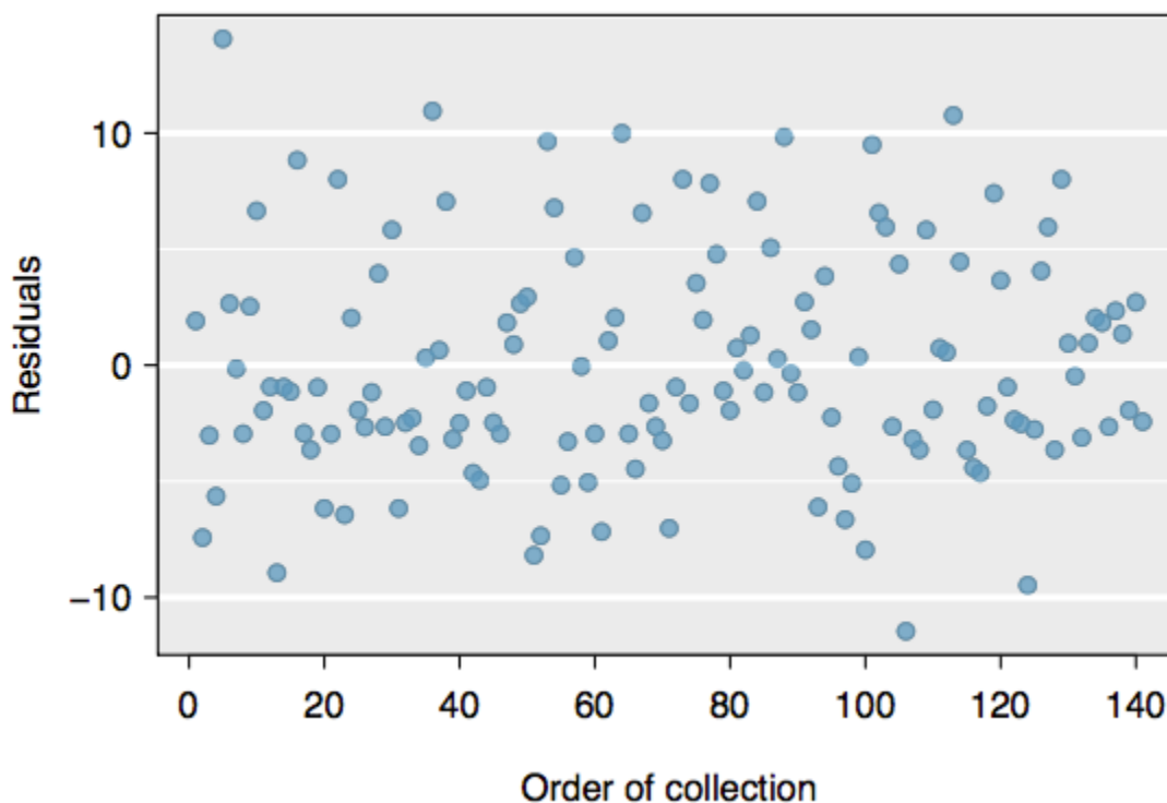
Figure 3. Plotting residuals in the order that their corresponding observations were collected helps identify connections between successive observations. If it seems that consecutive observations tend to be close to each other, this indicates the independence assumption of the observations would fail.
